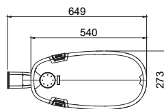
Luxis Square Small Coatingklasse: C3 Optioneel: C4 Montagemaat: 48 mm / 60 mm / 76 mm
