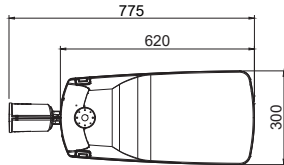
Luxis Square XS Coatingklasse: C3 Optioneel: C4 Montagemaat: 48 mm / 60 mm / 76 mm
